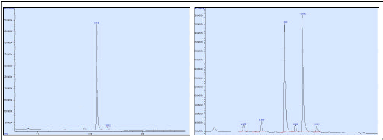
CHROMATOGRAMS OF CANNABIS SAMPLES reveal their chemical contents. Scale at left indicates amount detected in the sample. Scale at bottom is a measure of time as sample is heated from 200° to 325° during a 10-minute run of the gas chromatograph. As samples are heated, compounds separate and are detected at characteristic intervals. Chromatogram at left shows one sharp spike for THC and a very small one to its right for CBD. “This is what 99% of our chromatograms look like—high THC, almost no CBD,” says David Lampach. The chromatogram at right shows contents of Ganja Ma, a high-CBD strain for which no genetic material was preserved. Small spikes include one for CBN and three for compounds that Lampach says, “are unknowns, probably terpenoids, that we will be able to identify” when the lab is fully functional.
